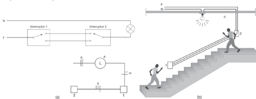
Figura 3.8 (a) Esquemas do three-way. (b) Exemplo do emprego do three-way.
